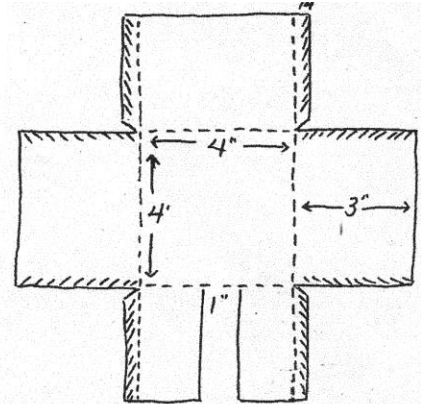
Plan for the lidless box
