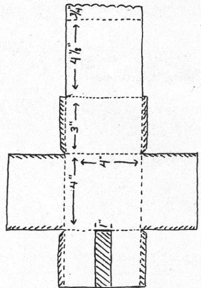
For an overlapping closure — all in one piece
